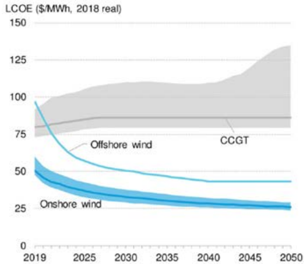
Wind vs coal and CCGT
