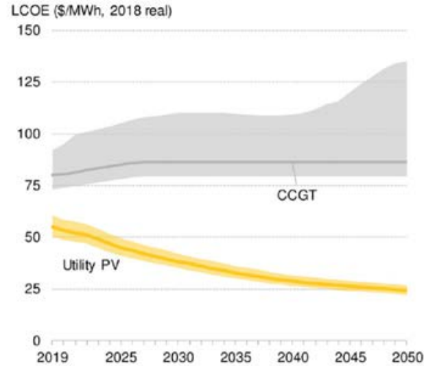
Utility-scale PV vs coal and CCGT
